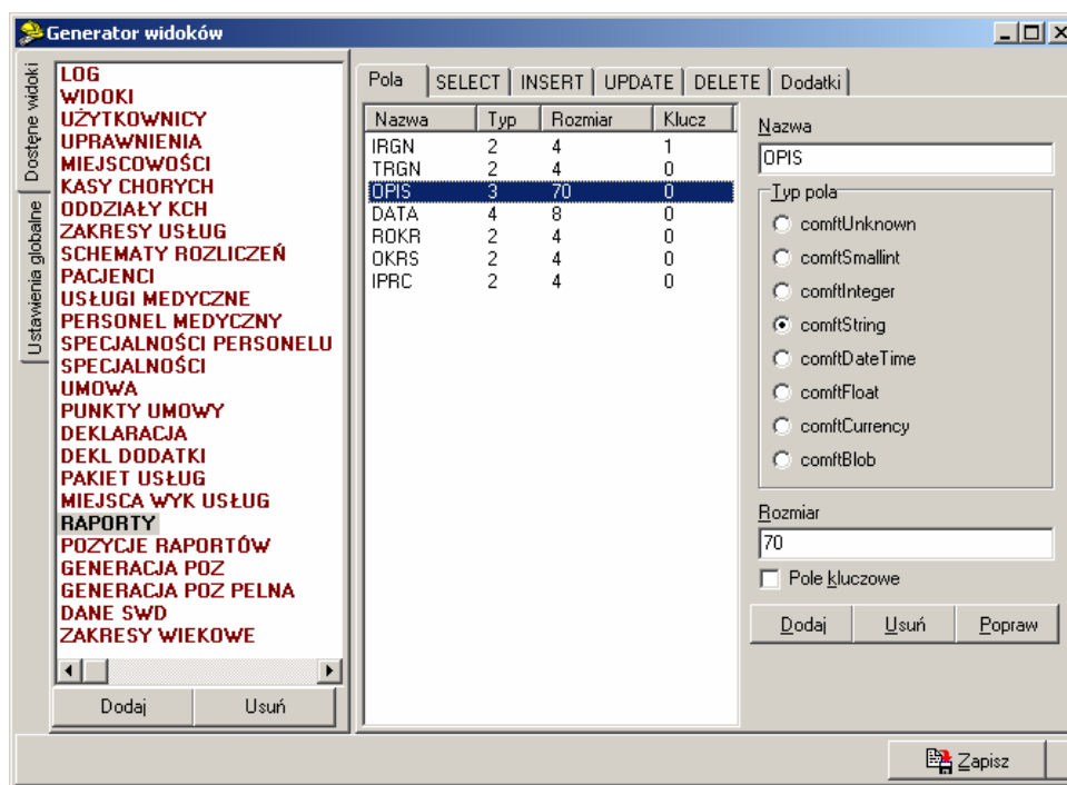
Rys. 2. Program VGEN
